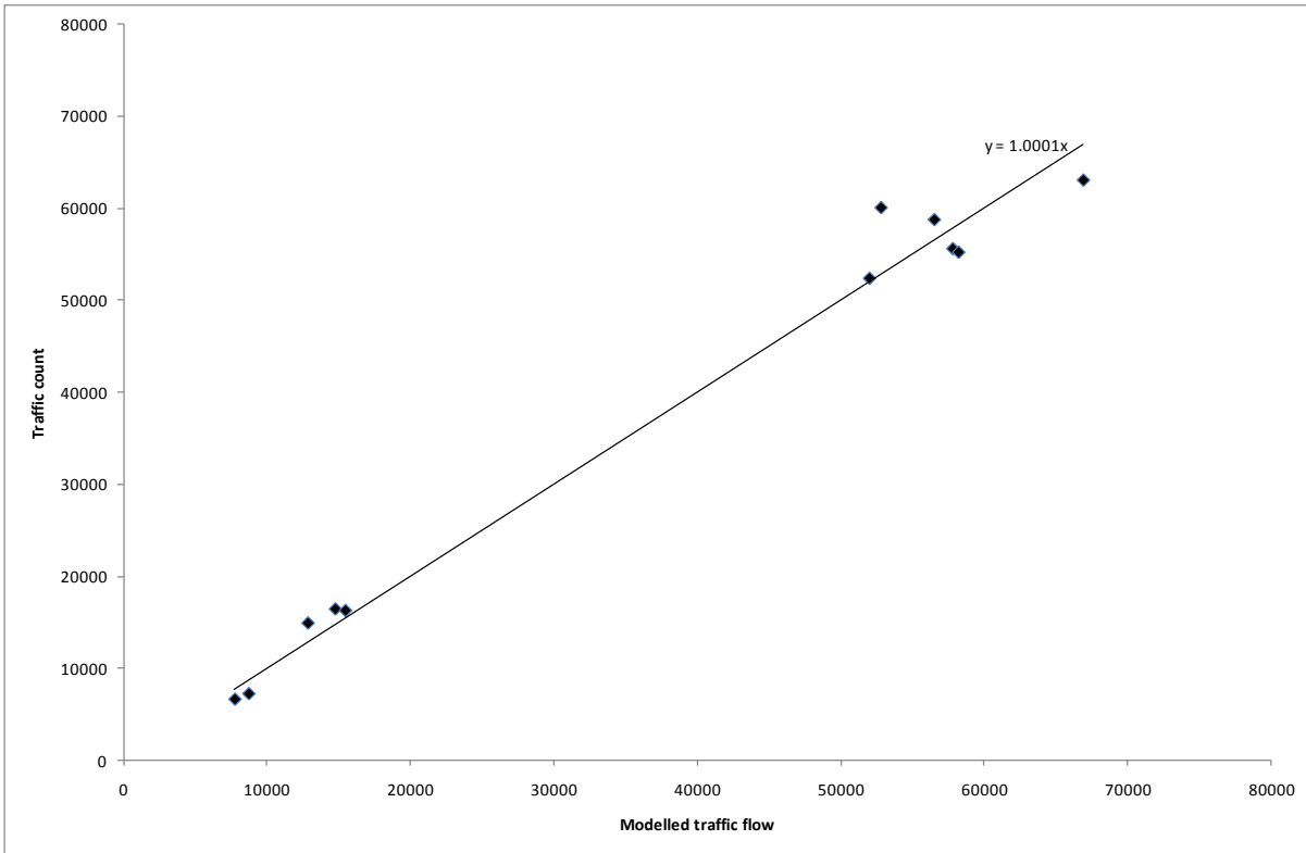
Fig. 3: Comparison of modelled traffic estimates with actual counts for motorways
