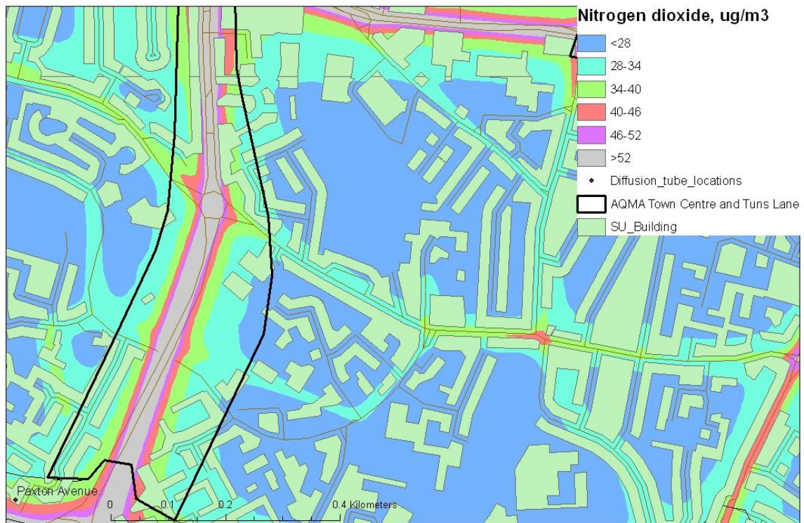
Fig.11: Predicted concentrations for 2009 in the south part of the Tuns Lane AQMA
