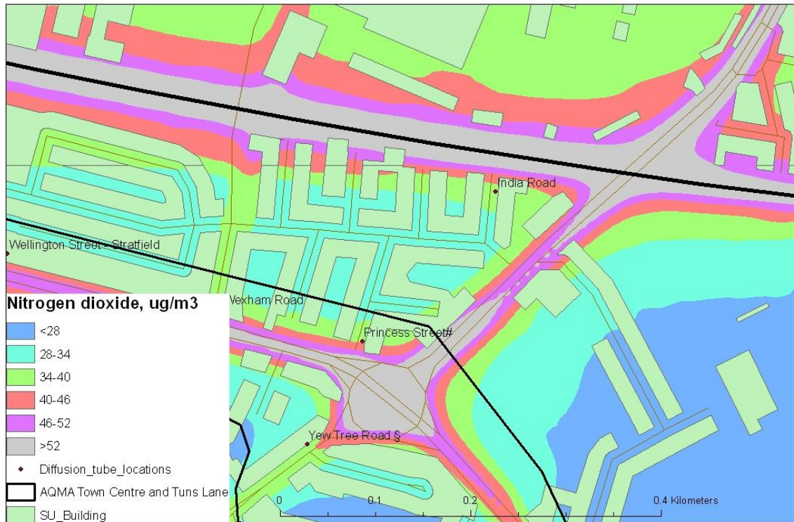
Fig. 14: Modelled concentration in the region of the India Road monitoring site
