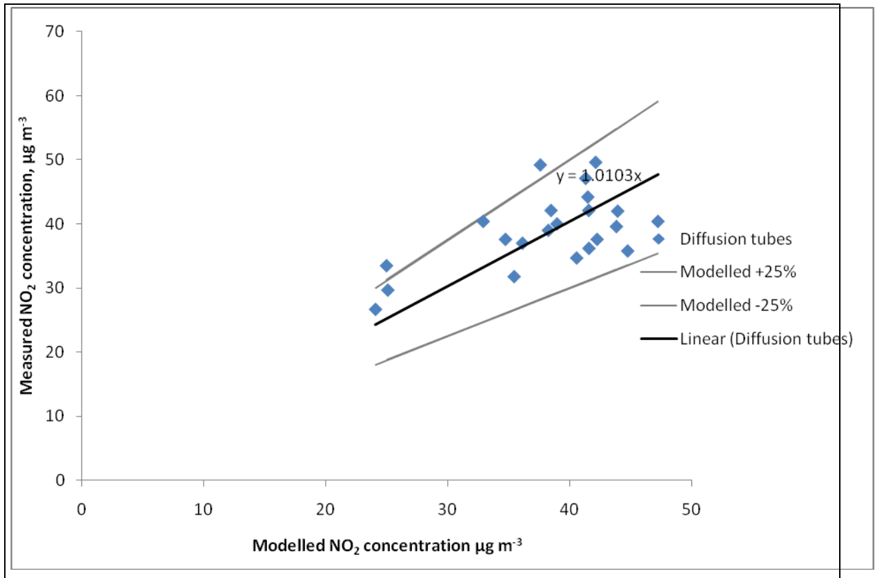
Fig. 8 : Comparison of modelled and measure nitrogen dioxide concentrations
