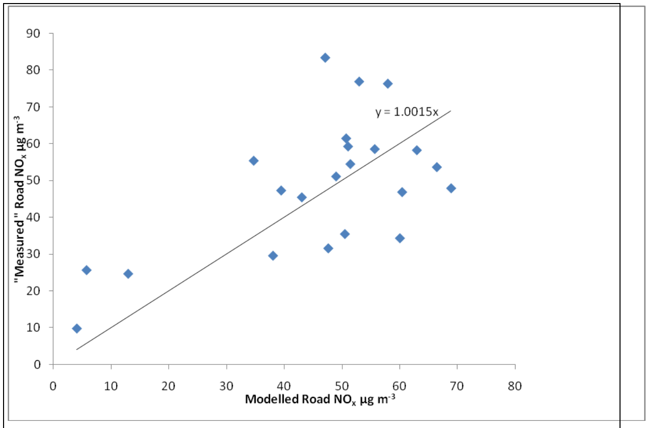
Fig. 7: Comparison of modelled and measured oxides of nitrogen concentrations
